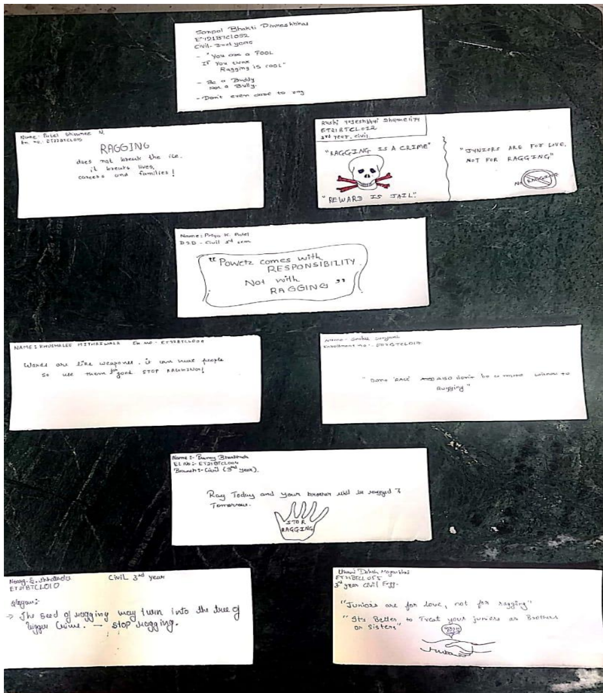
Figure 7: Selective slogans
